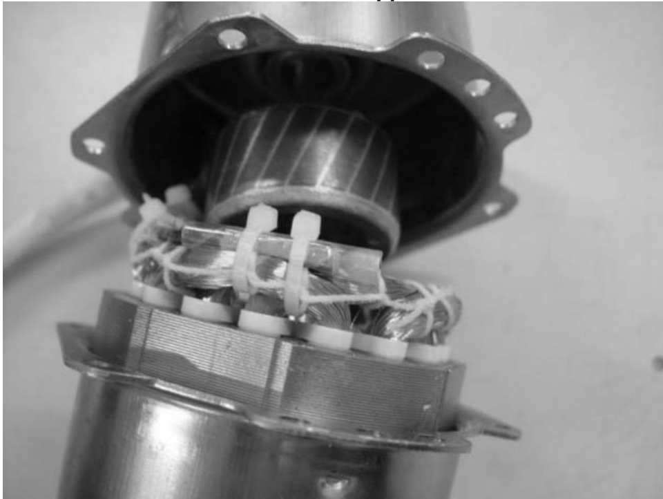
Position of thermal motor protector
