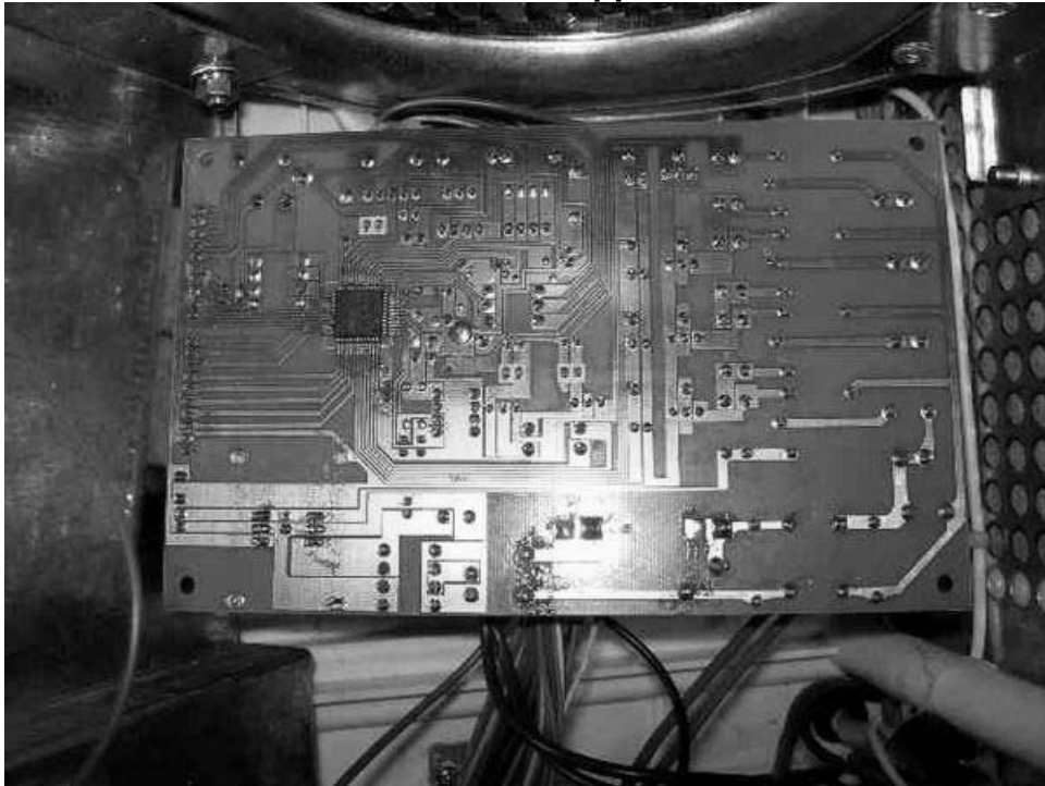
Routing side of main PCB of B-767 and B-777
